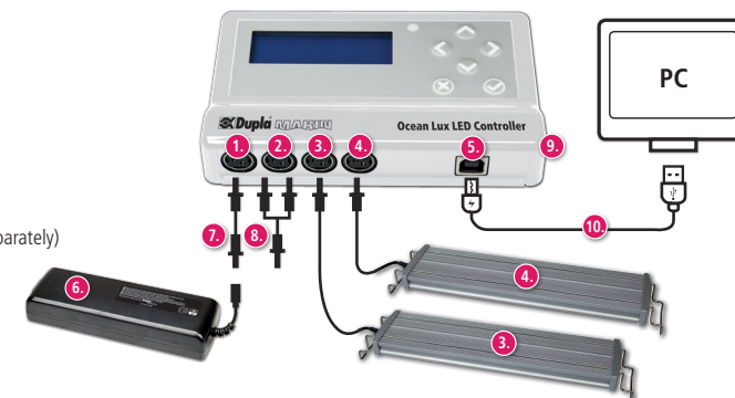
Connecting cable
