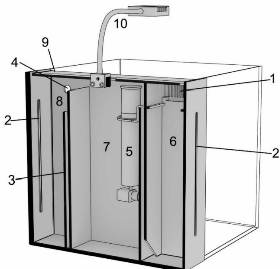
Fig. 1: Filter with suspended skimmer
